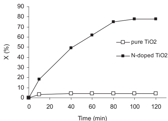
Fig. 8. The degree of photocatalytic degradation (X) as a function of irradiation time at 587 nm for pure \text{TiO}_2 ( \square ) and Nitrogen doped \text{TiO}_2 ( \blacksquare ).
